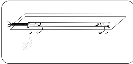
5. Fix the bottom shell to the wall with tools
