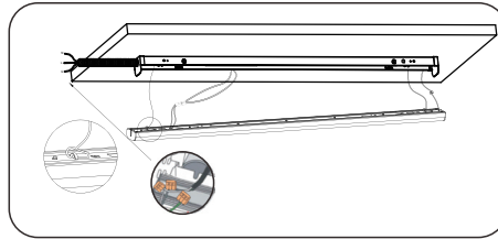
6. Hook the lamp cover with safety wire and plug in the plug-in terminal and ground terminal, Connect the wires: AC/L match black; AC/N match white; PC/green match ground
