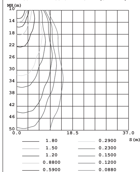
CO PLANE ISOLUX DIAGRAM (UNIT: lx)
