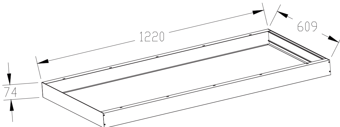
TLPBL24WMF Surface mount frame 2' x 4' (609 mm x 1220 mm)
