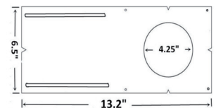
TLMP4 4" installation plate
